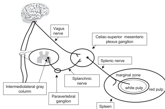
Fig. 7. Anatomical basis of the cholinergic antiinflammatory pathway. Two-neuron model of vagus nerve modulation of cytokine production via the splenic nerve: The preganglionic neuron originates in the dorsal motor nucleus of the vagus; the postganglionic neuron, located in ganglia of the celiac-superior mesenteric plexus, reaches the spleen through the splenic nerve.
